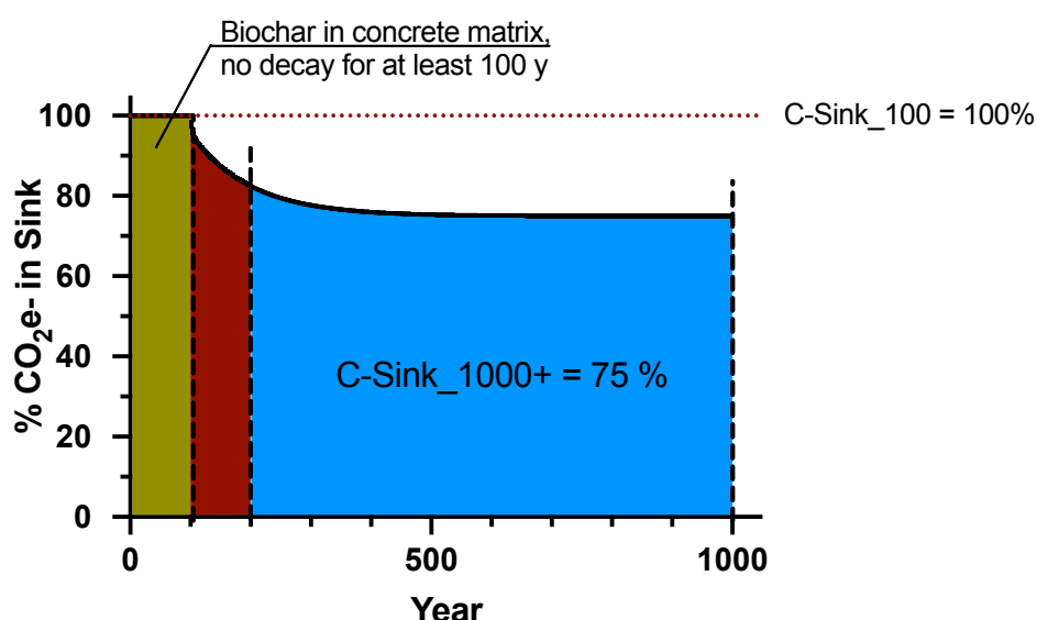
Figure 3: C-sink curve of concrete embedded biochar with an H/Corg ratio < 0.4. The PAC fraction is registered with a persistence of > 1000 years. The SPC fraction is registered without decay for 100 years. After 100 years, the concrete embedded biochar is conservatively considered as if applied to soil independent of the recycling or landfill deposition scenario. The C-Sink 100 of a construction C-Sink is 100% and the C-Sink 1000+ is 75.0%.
